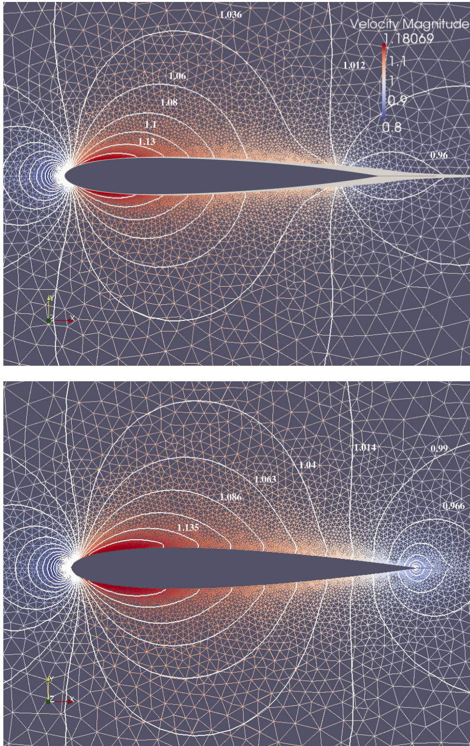
Figure 21: Mesh and velocity contours around a NACA0012 airfoil. Viscous-inviscid flow (top) and inviscid flow (bottom). Velocity distribution in m.s^{-1}
