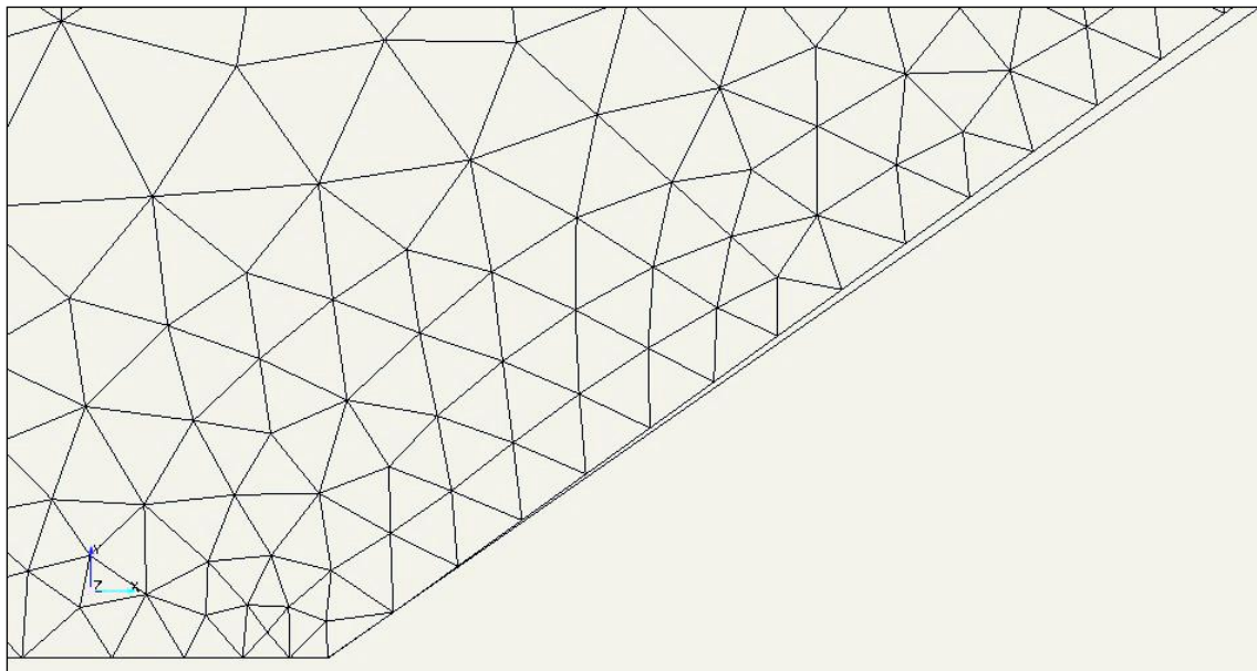
Figure 15: Mesh movement on the \beta=0.4 slope mesh, magnified 30 times
