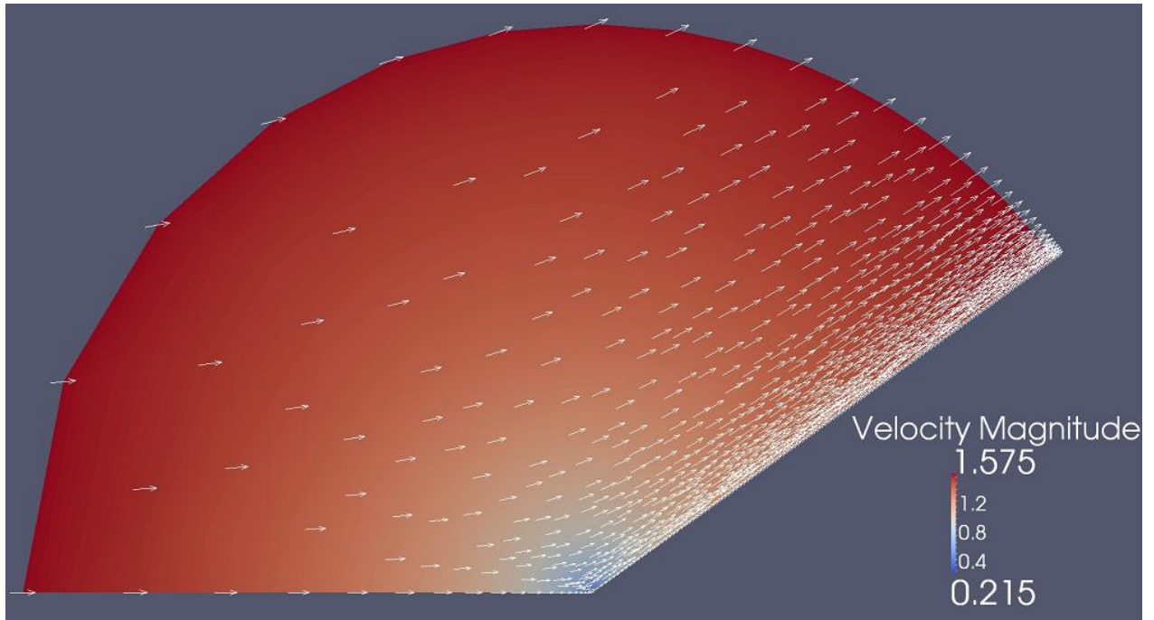
Figure 14: Velocity distribution in m.s^{-1} for the entire flow field ( \beta=0.4 )
